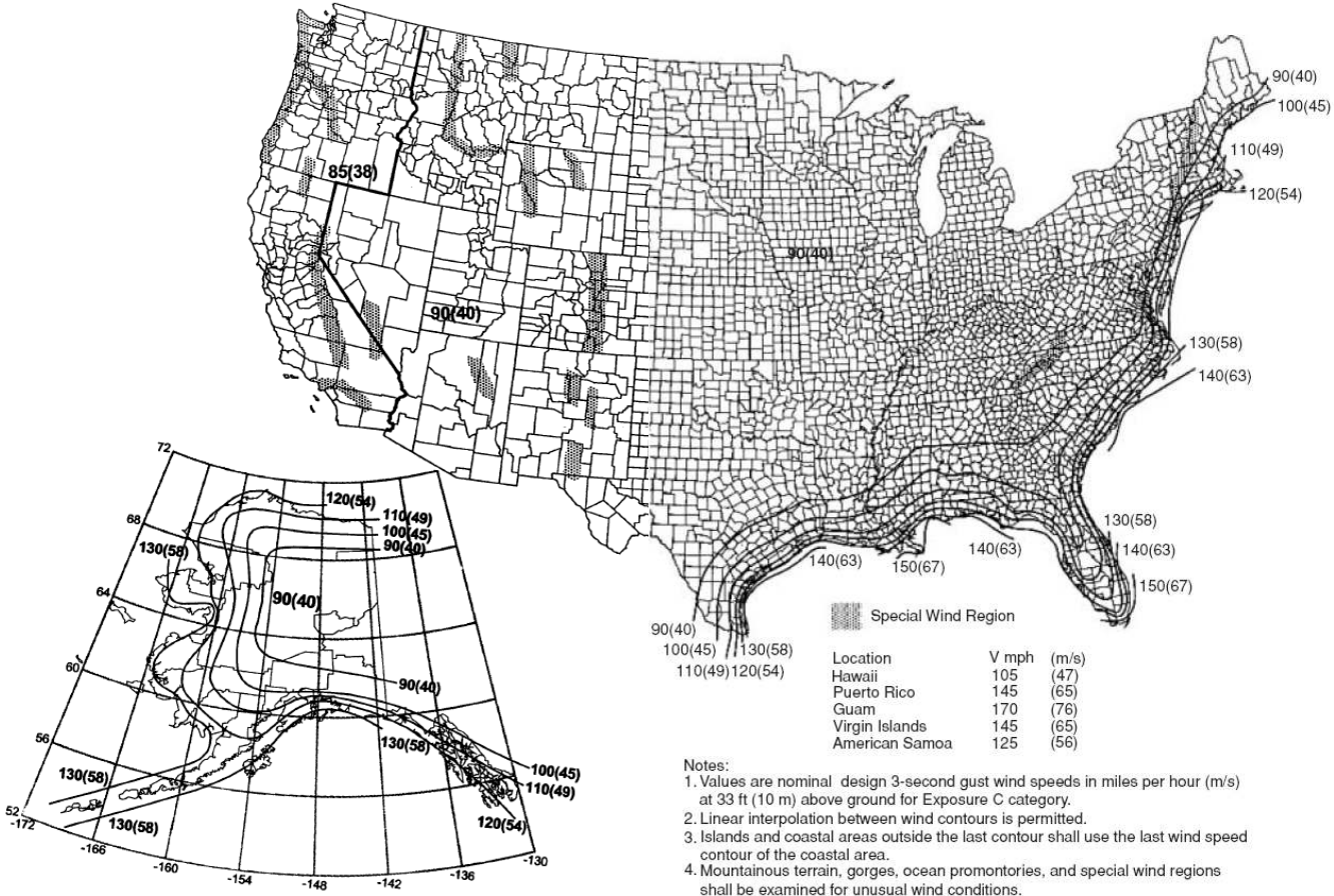
FIGURE 6-1 continued BASIC WIND SPEED
